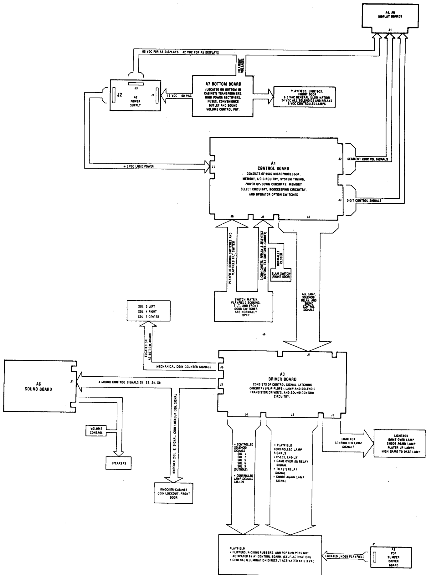
SYSTEM 80 BLOCK DIAGRAM
